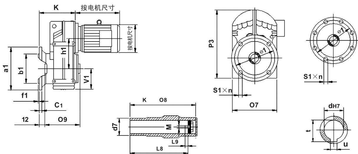
(FA法兰安装 FA Flange-mounted)
